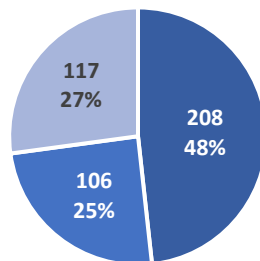
Response Distribution
