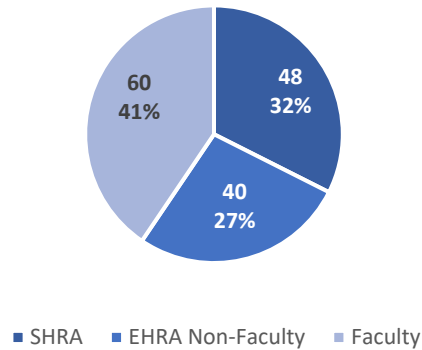
Response Distribution
